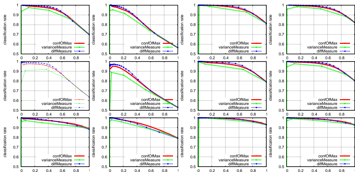
Figure 12. Classification rates for \theta_{\text{conf}} in the range of [0, 1] for different descriptors and confidence measures using an MLP. The first row shows the VFH descriptor accuracies for ToF sensors in an angle of 30^\circ , respectively in an angle of 90^\circ for the second row. The third row concerns the ESF descriptor for an angle of 30^\circ between the two sensors. From left to right, the first two columns show the performance when using only the first or second ToF sensor; the third column represents the late fusion approach and the fourth column the early fusion approach.
